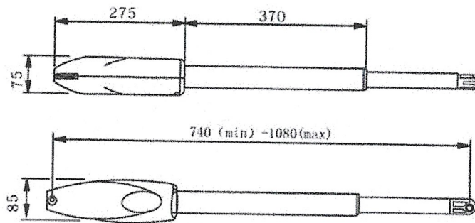
Nomenclature of Swing Gate Motor
